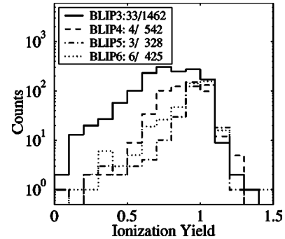
FIG. 23. Distributions of ionization yield Y for veto-anticoincident single-scatter events with recoil energies between 10–100 keV, fully contained in the inner electrode of BLIP 3 (solid line), BLIP 4 (dashed line), BLIP 5 (dotted-dashed line), or BLIP 6 (dotted line). BLIP 3's high event rate, particularly for yields slightly too high to be nuclear recoils ( Y \approx 0.5 ), indicates its contamination by a source of low-energy electrons. Although BLIP 4 shows a high rate of events with Y \approx 0.8 , its rate just above the nuclear-recoil acceptance region is similar to that of BLIP 5 and BLIP 6. The legend lists the number of events that fall in the nuclear-recoil acceptance region for each detector as a fraction of the total number of events in that detector.
