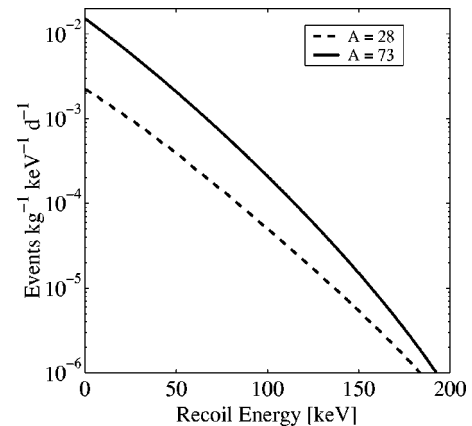
FIG. 42. Expected differential recoil-energy spectra for Si ( A=28 ) and for Ge ( A=73 ), for a 100-GeV/ c^2 WIMP with WIMP-nucleon cross section \sigma=10^{-42} cm 2 under standard assumptions listed in Sec. VI A.
