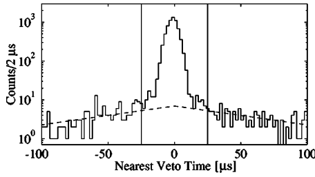
FIG. 21. Distribution of the nearest veto-trigger times for phonon-trigger events, relative to the time of the ionization pulse, for events above the ionization-search threshold. The width of the peak is dominated by the uncertainty on the reconstructed time of the ionization pulse. The exponential accidental distribution is shown as dashes. The \pm 25\text{-}\mu\text{s} coincidence window is indicated.
