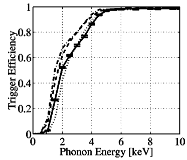
FIG. 16. Efficiency of hardware phonon trigger vs. phonon energy E_P , for BLIP 3 (solid line), BLIP 4 (dashes), BLIP 5 (dotted-dashes), and BLIP 6 (dots). Statistical uncertainty ( 1\sigma ), shown for BLIP 3, is similar in the other detectors. These results are averaged over the entire data set; the slight residual trigger inefficiency above 5 keV is dominated by a four-week period with slightly worse trigger filters.
